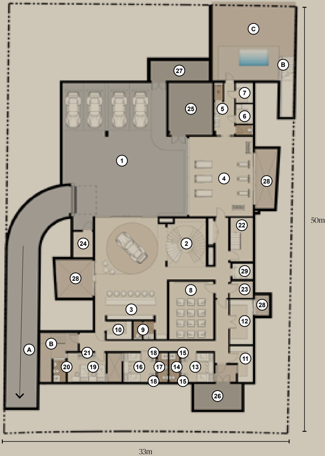
BASEMENT FLOOR
