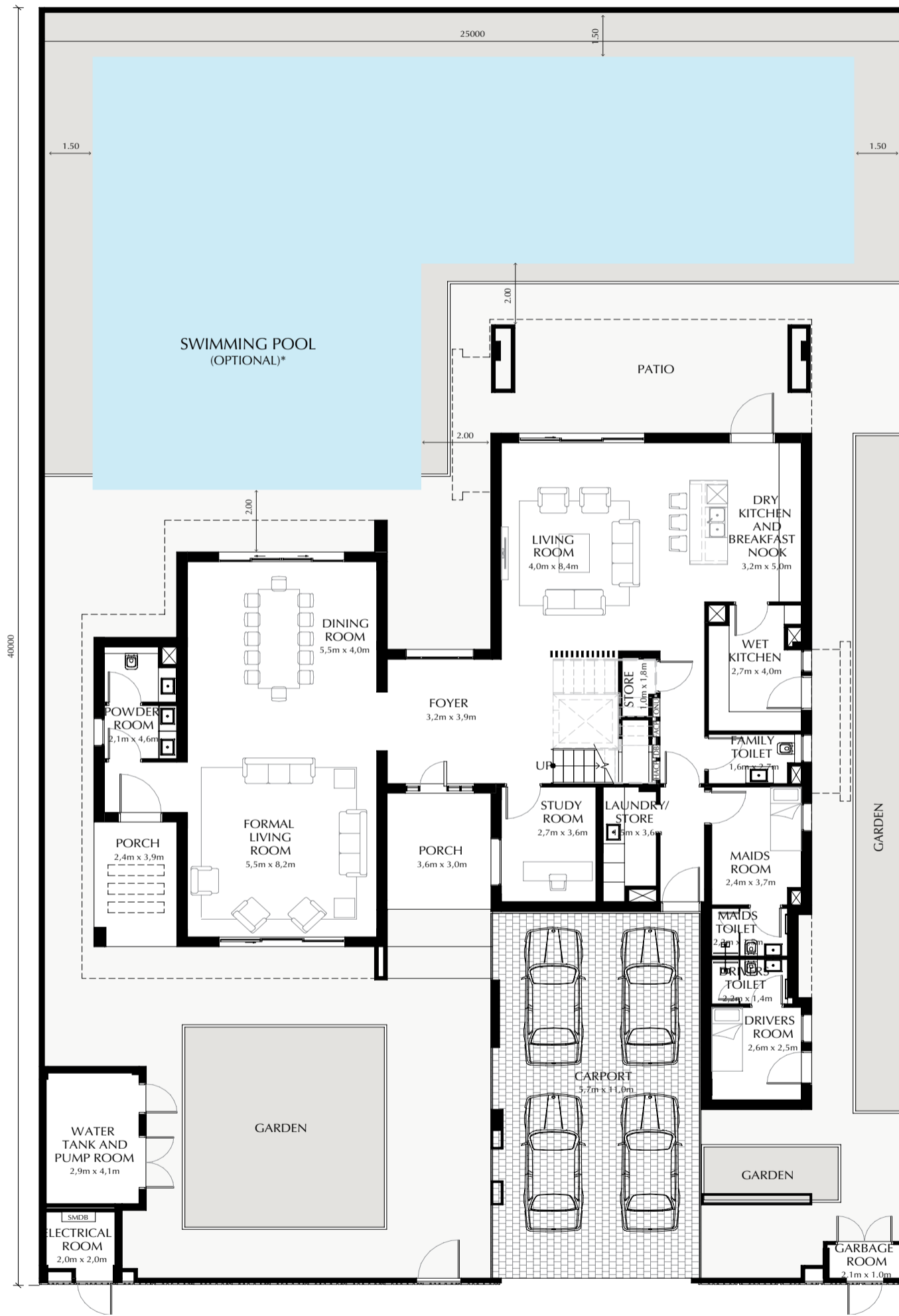
Ground Floor
