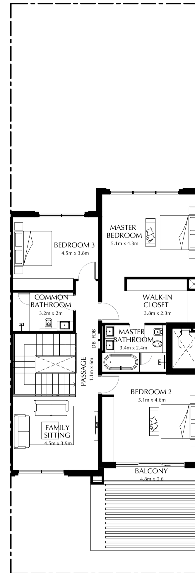
First Floor
