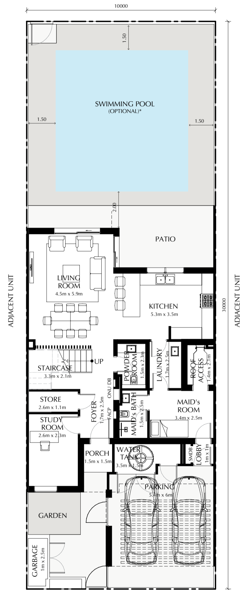
Ground Floor
