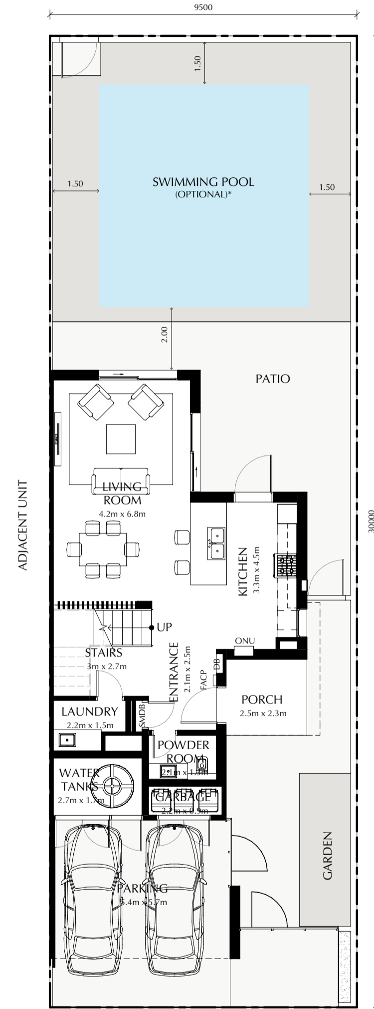
Ground Floor
