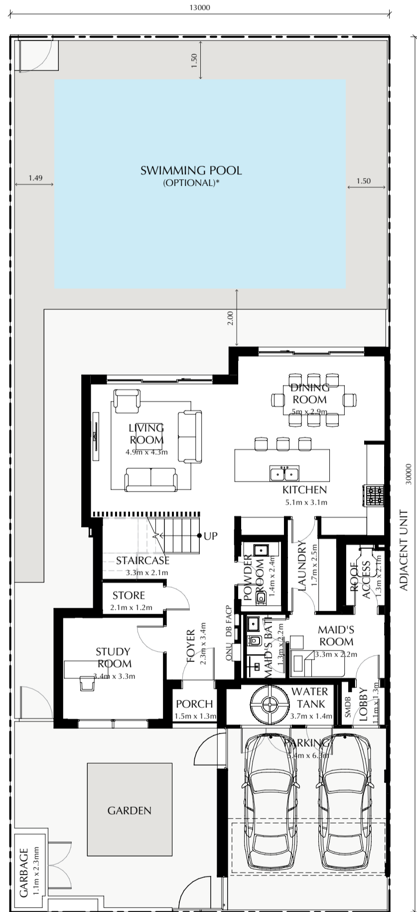
Ground Floor
